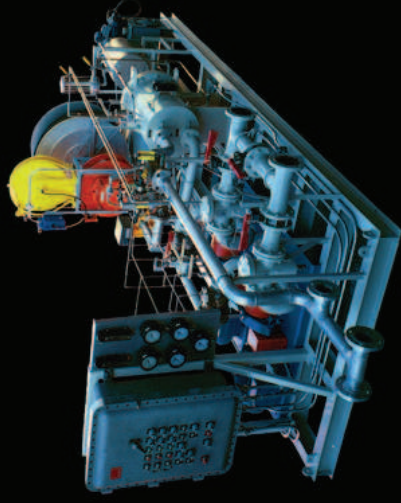
Marine One Fueling Skid Camp David, MD
